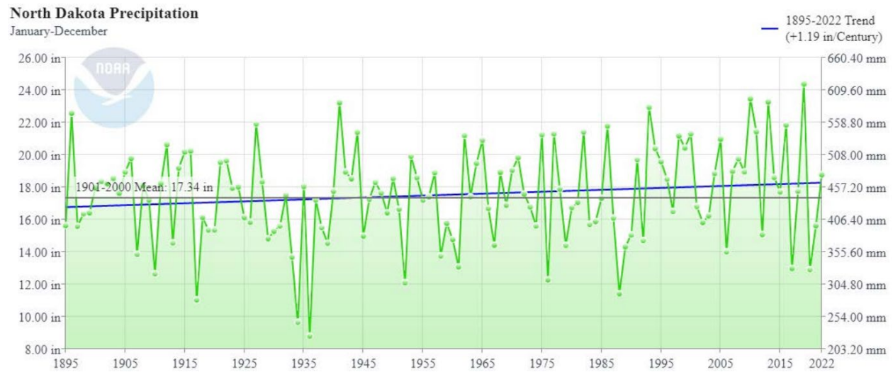
Figure 10: Observed Total Annual Precipitation for North Dakota from 1895 to 2021 76
